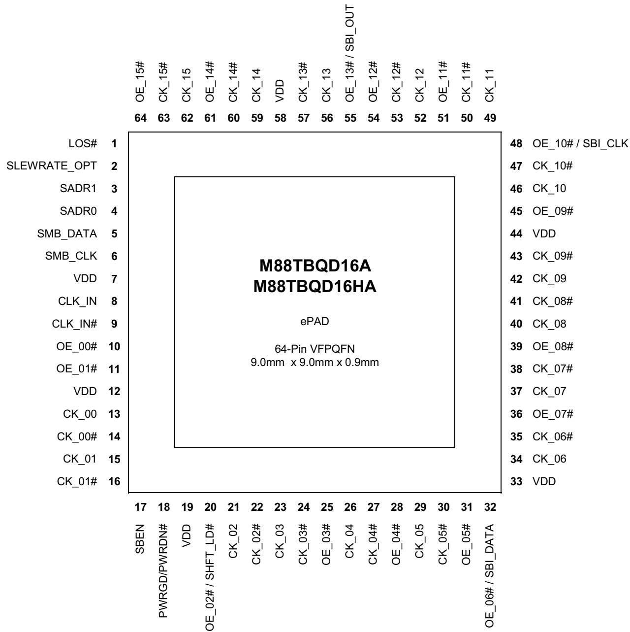
Figure 3. M88TBQD16 Pin Assignment
