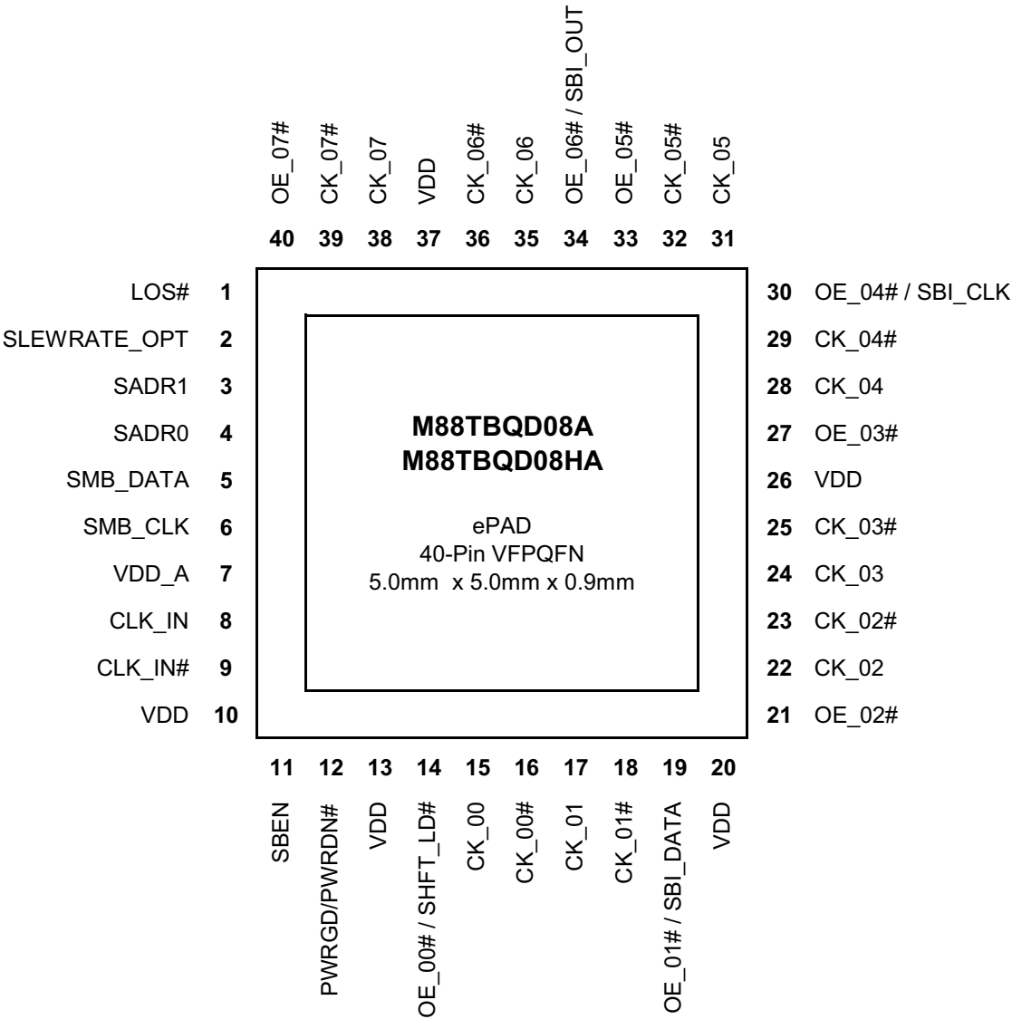
Figure 5. M88TBQD08 Pin Assignment
