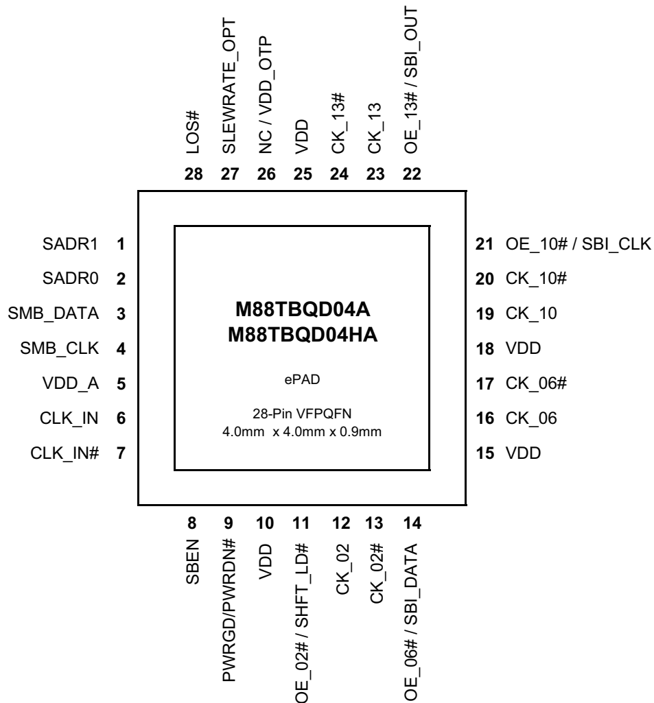
Figure 6. M88TBQD04 Pin Assignment
