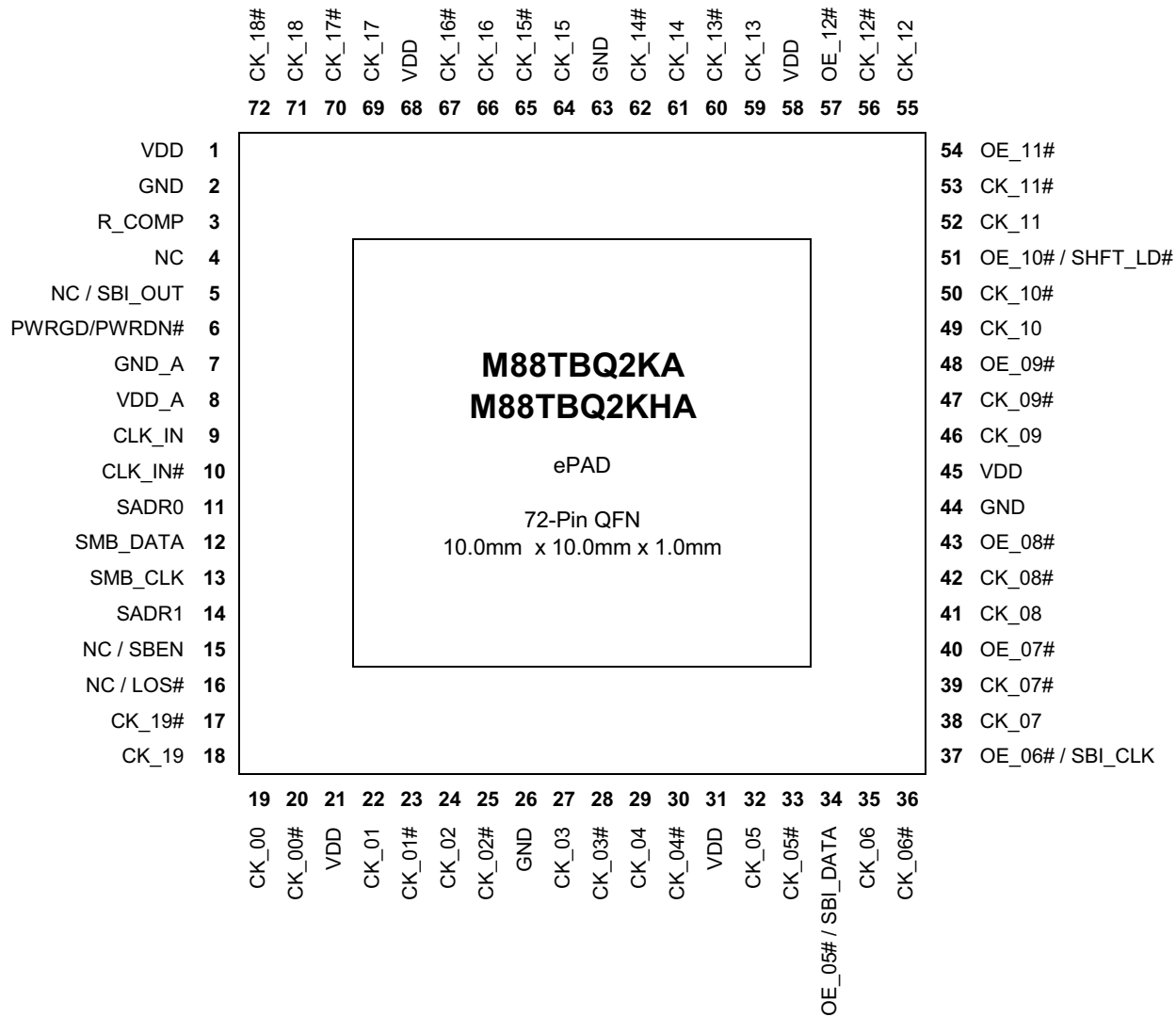
Figure 1. M88TBQ2K Pin Assignment
